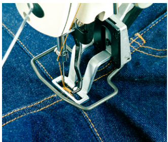
LK-1900S-H type (Bartacking crotch of jeans)
